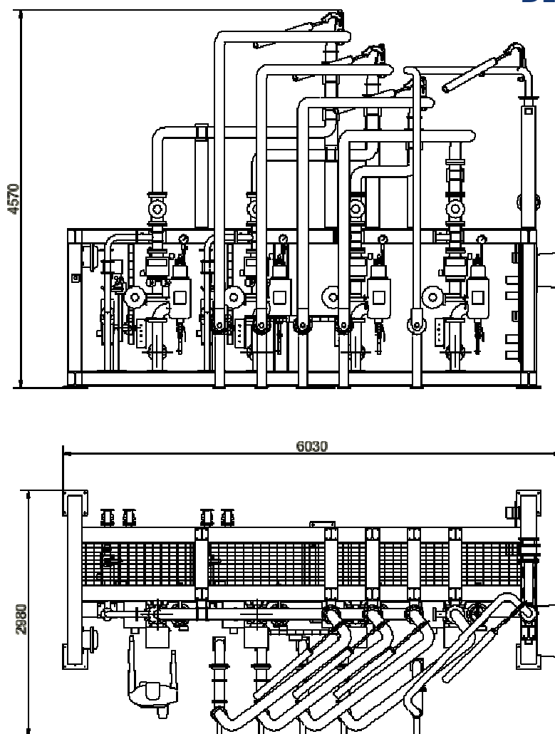
4 loading arms + vapor recovery skid general dimensions.
